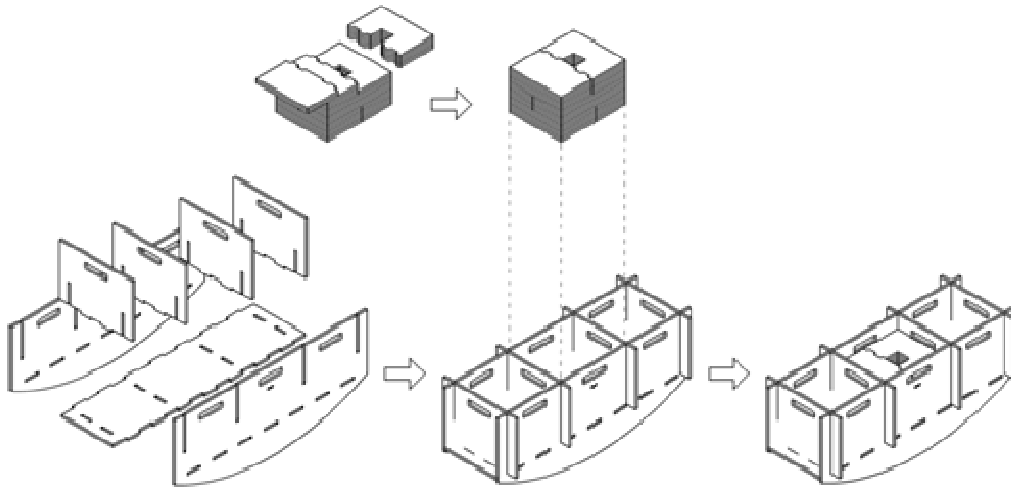
Fig. 5: Cradle assembly system.
