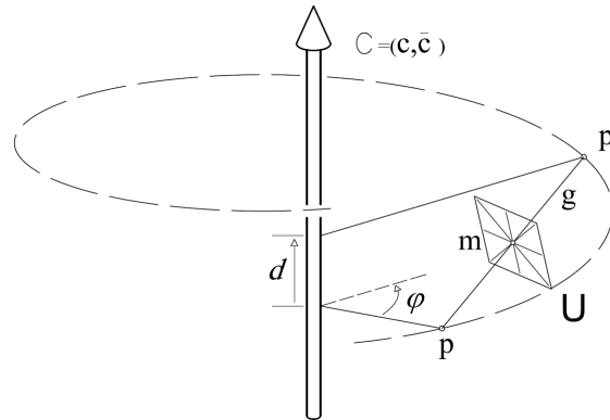
Fig. 2: The bisecting plane between two positions of a point.
