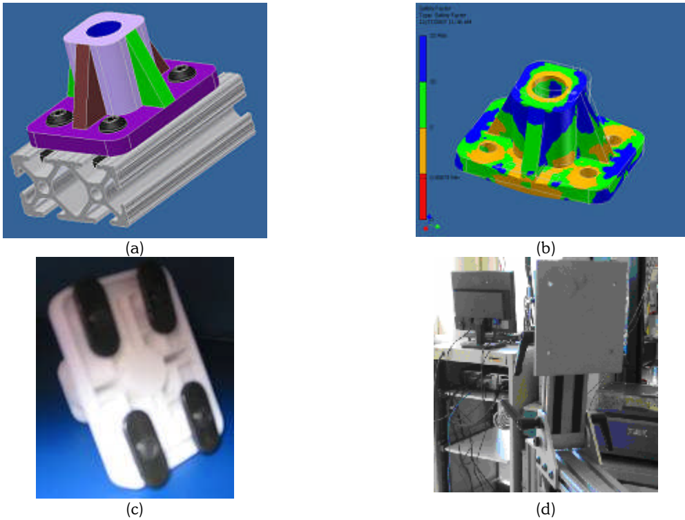
Fig. 5: Product design course examples: (a) 80/20® extrusion and ABS plastic lamp holder (CAD); (b) FEA analysis of lamp holder; (c) photograph of rapid prototyped lamp holder; (d) photograph of LCD NEMA monitor holder.
