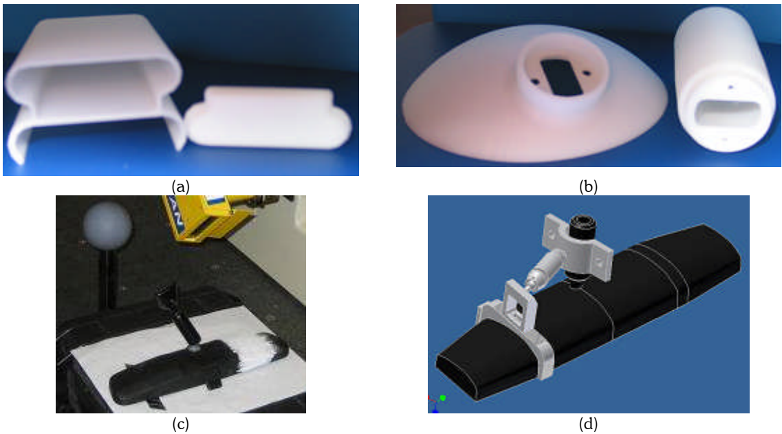
Fig. 6: Product design course examples: (a) iPod® ear bud holder; (b) central vacuum bug attachment; (c) automobile rear view mirror laser scanning; (d) automobile rear view mirror holder stabilizer (CAD).
