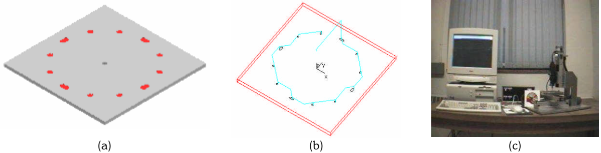
Fig. 4: CNC machining example: (a) solid model; (b) tool path planning; (c) Dremel® tool and stepper motor based online machine.
