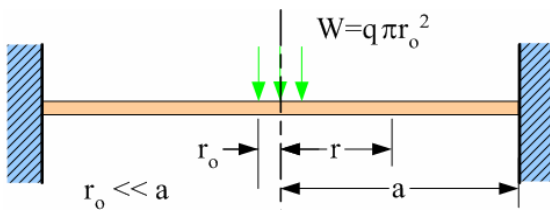
Fig. 7: A clamped circular plate under distributed body force [18].
