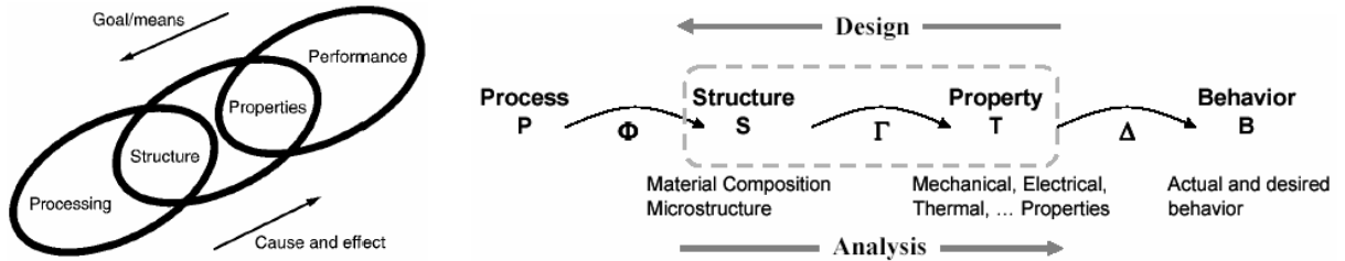
Fig. 11: Systematic design framework: (left) three-link chain model for materials science and engineering [22]; (right) Process-Structure-Property-Behavior model for design for additive manufacturing [4].
