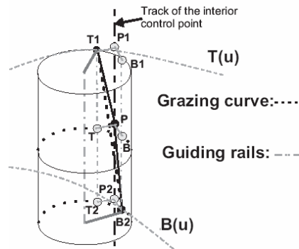
Fig. 3: A grazing curve and its control points on a cylindrical tool.
