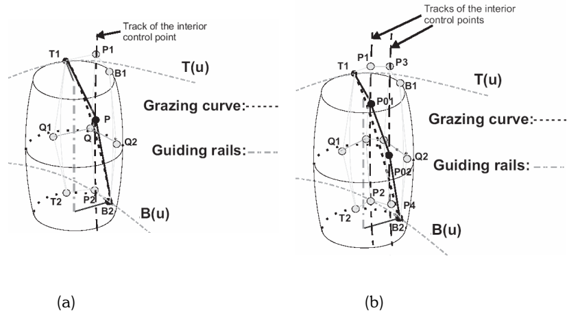
Fig. 11: Grazing curve and its control points on a tool of revolution (a) one track (b) two tracks.
